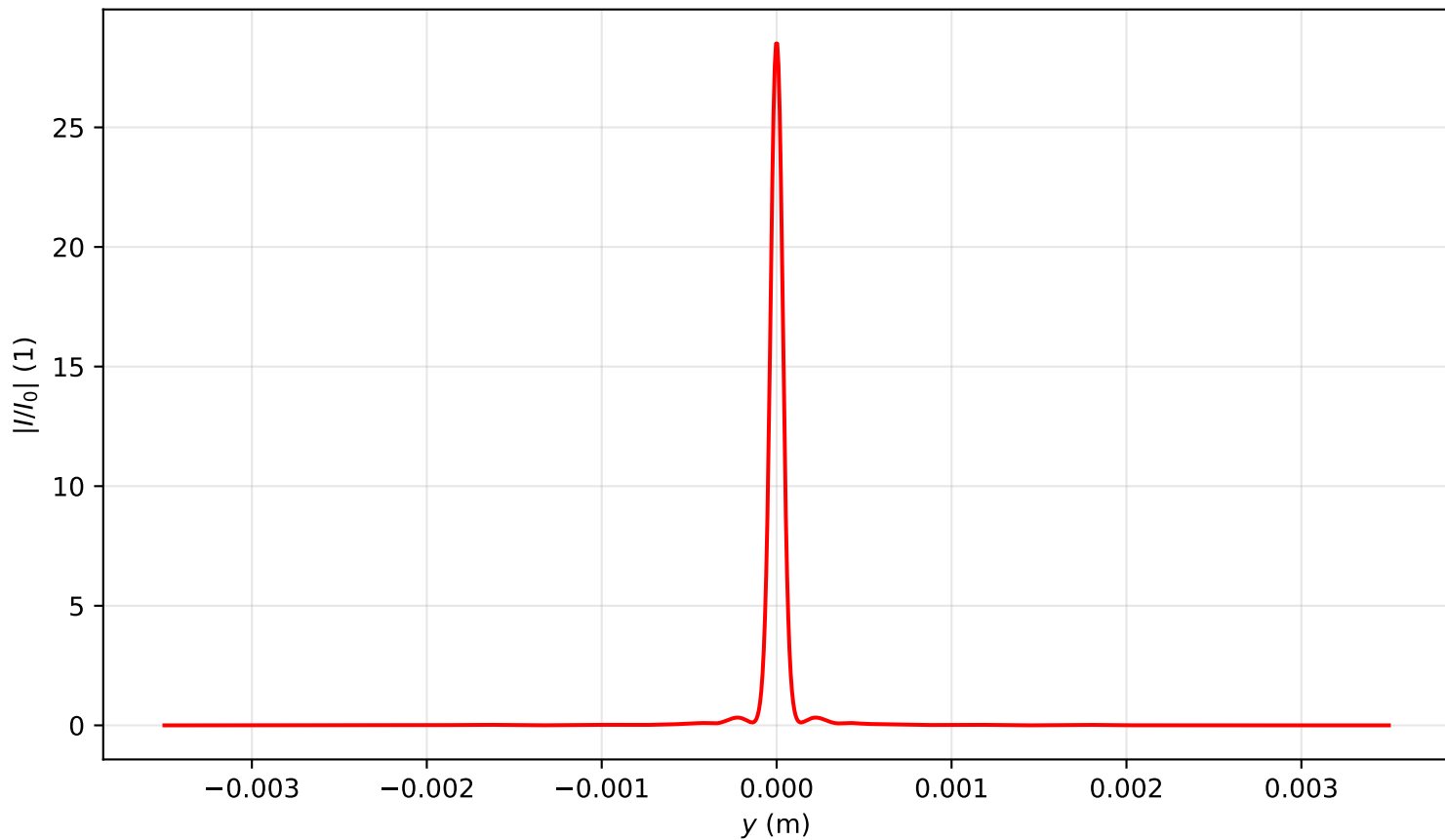
Intensity profile I(x=0, y, z=2.388)/I_0 , P_{in}=3.5P_{cr} , artificial time
